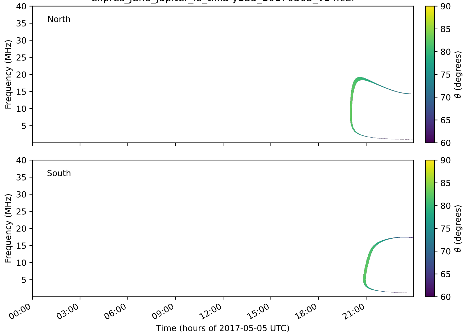
expres_juno_jupiter_io_txka-y235_20170505_v14.cdf
