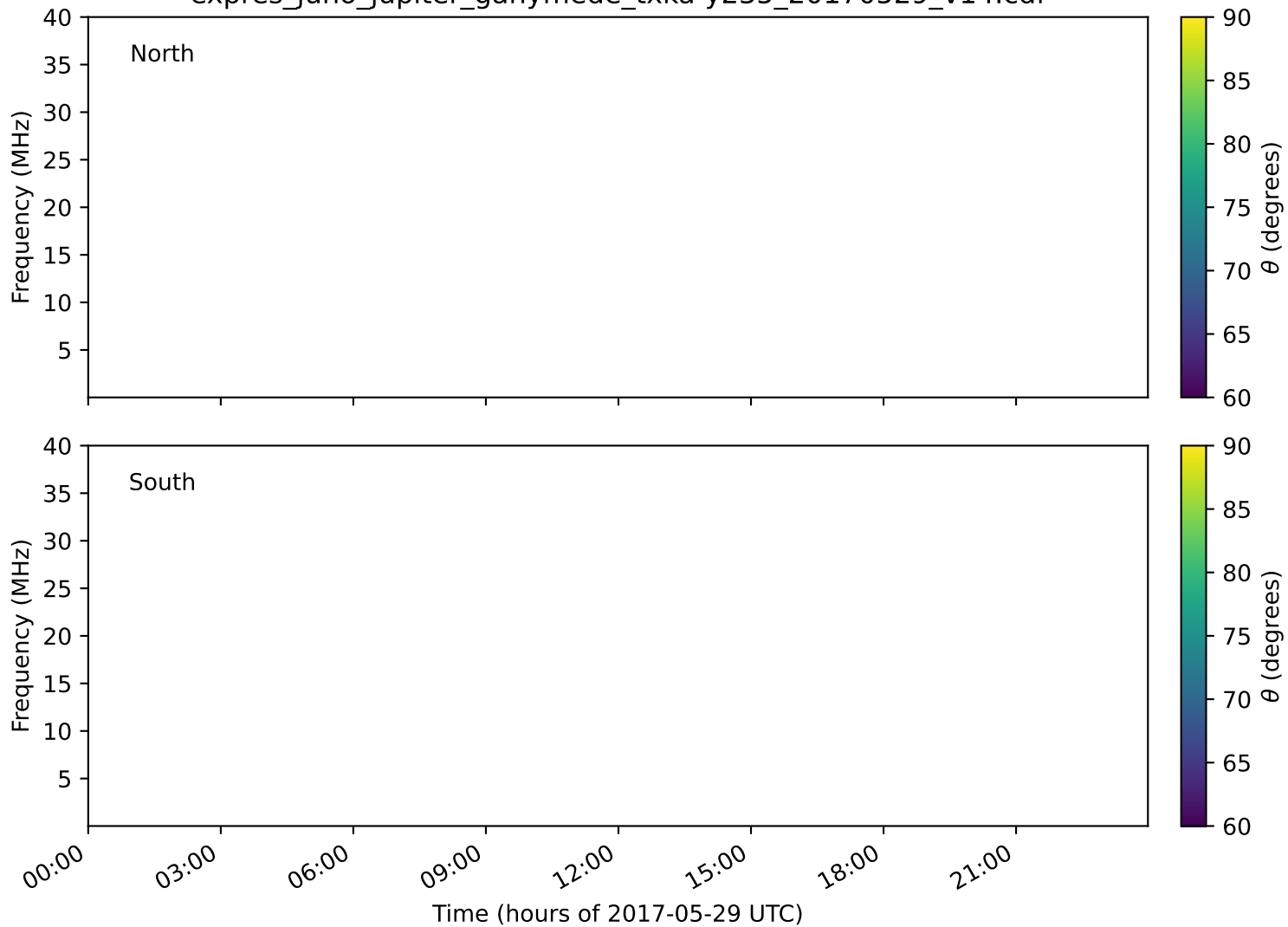
expres_juno_jupiter_ganymede_txka-y235_20170529_v14.cdf
