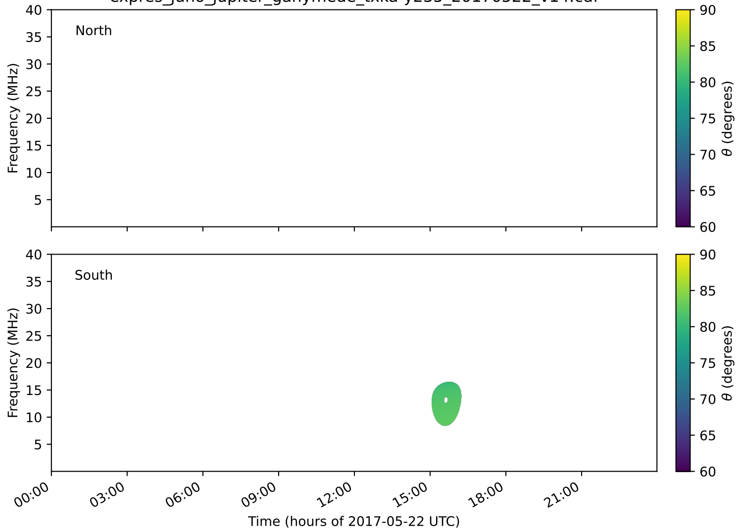
expres_juno_jupiter_ganymede_txka-y235_20170522_v14.cdf
