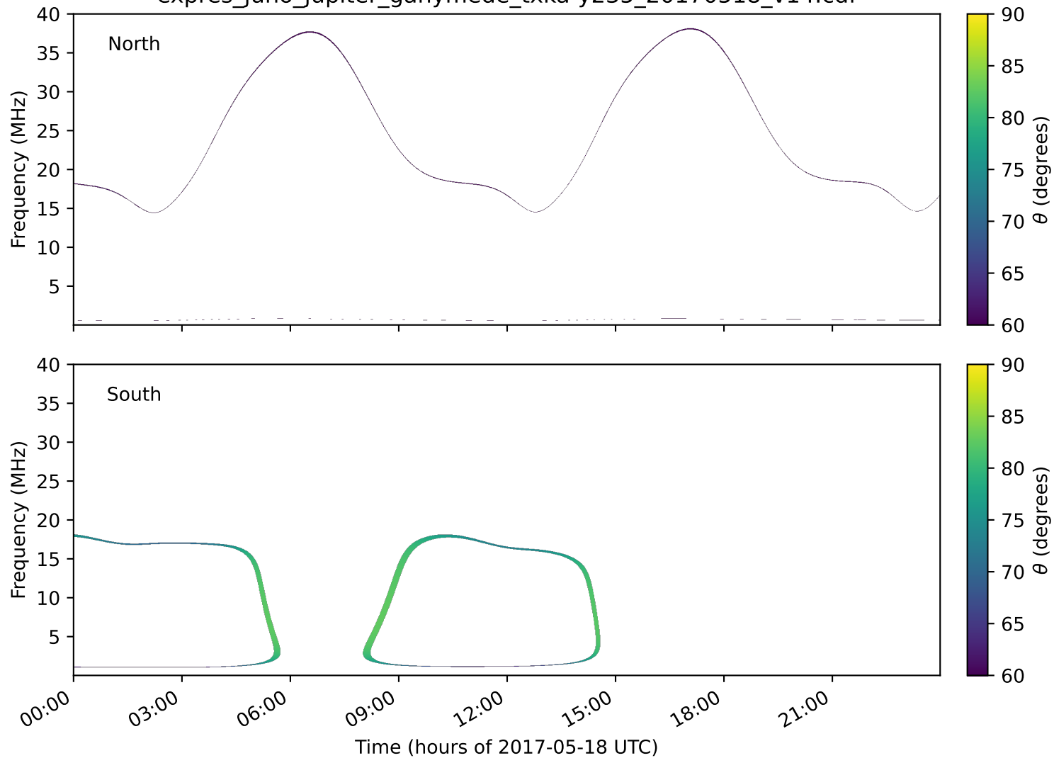
expres_juno_jupiter_ganymede_txka-y235_20170518_v14.cdf
