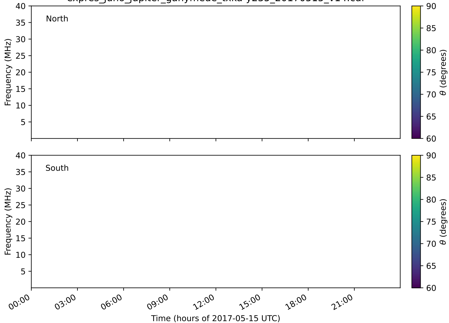
expres_juno_jupiter_ganymede_txka-y235_20170515_v14.cdf
