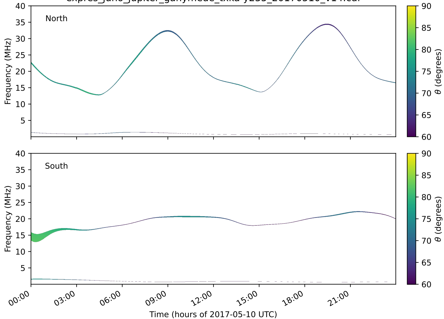
expres_juno_jupiter_ganymede_txka-y235_20170510_v14.cdf
