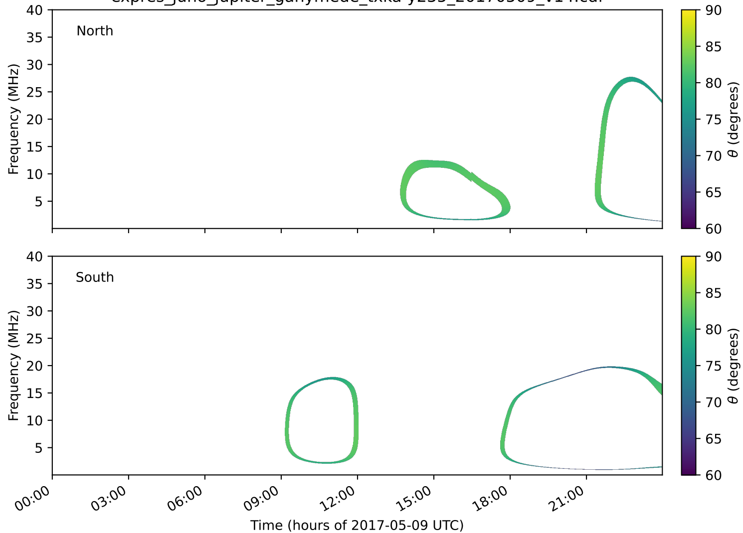
expres_juno_jupiter_ganymede_txka-y235_20170509_v14.cdf
