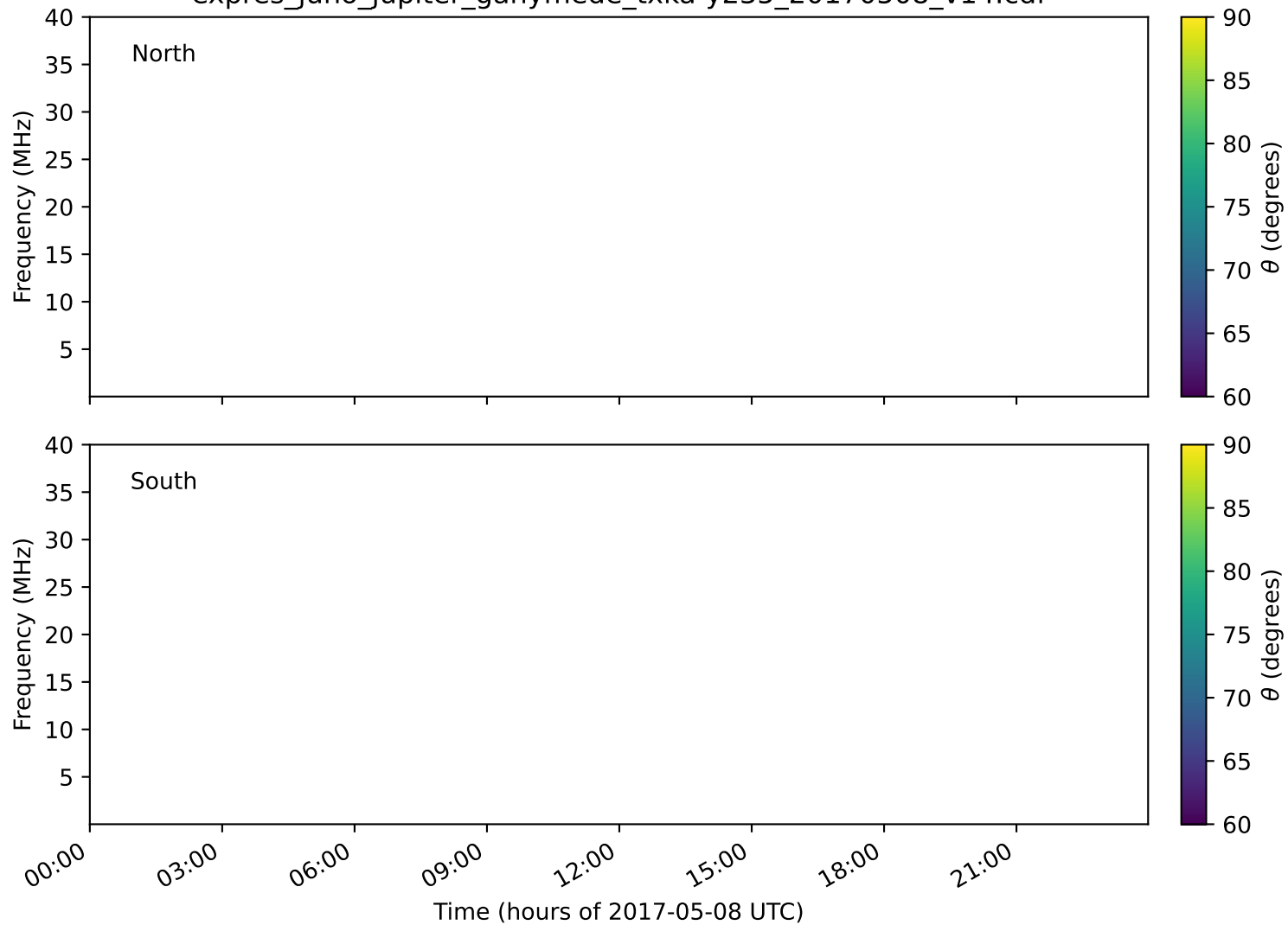
expres_juno_jupiter_ganymede_txka-y235_20170508_v14.cdf
