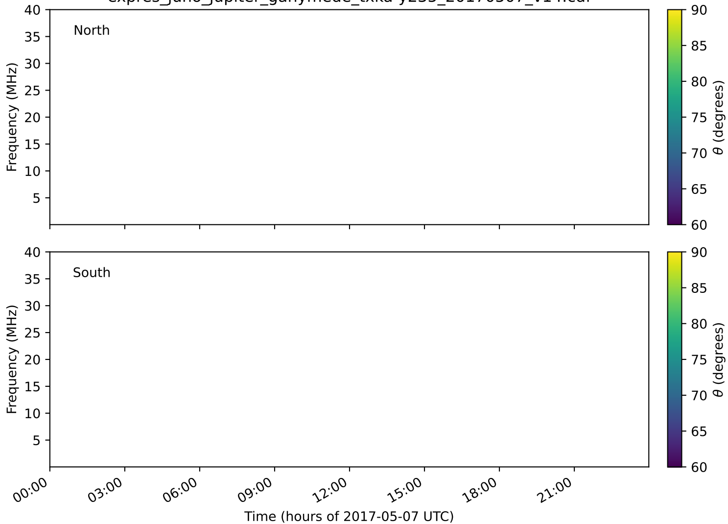
expres_juno_jupiter_ganymede_txka-y235_20170507_v14.cdf
