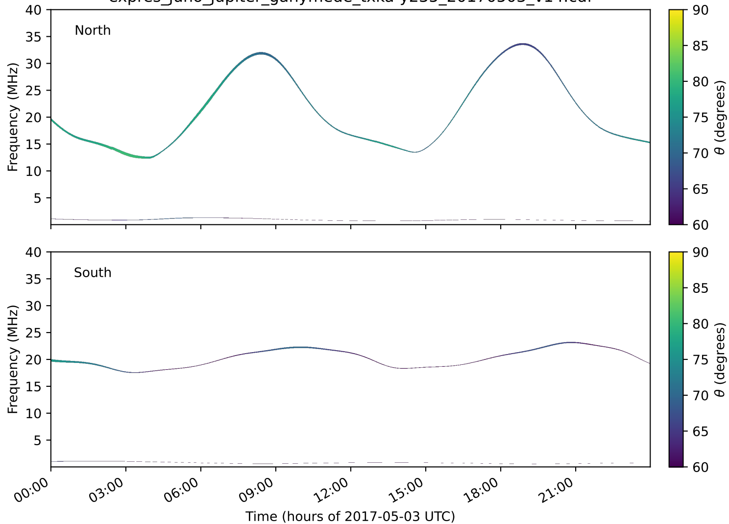
expres_juno_jupiter_ganymede_txka-y235_20170503_v14.cdf
