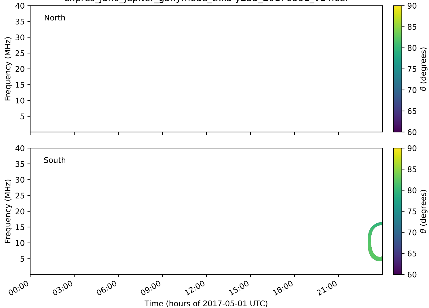
expres_juno_jupiter_ganymede_txka-y235_20170501_v14.cdf
