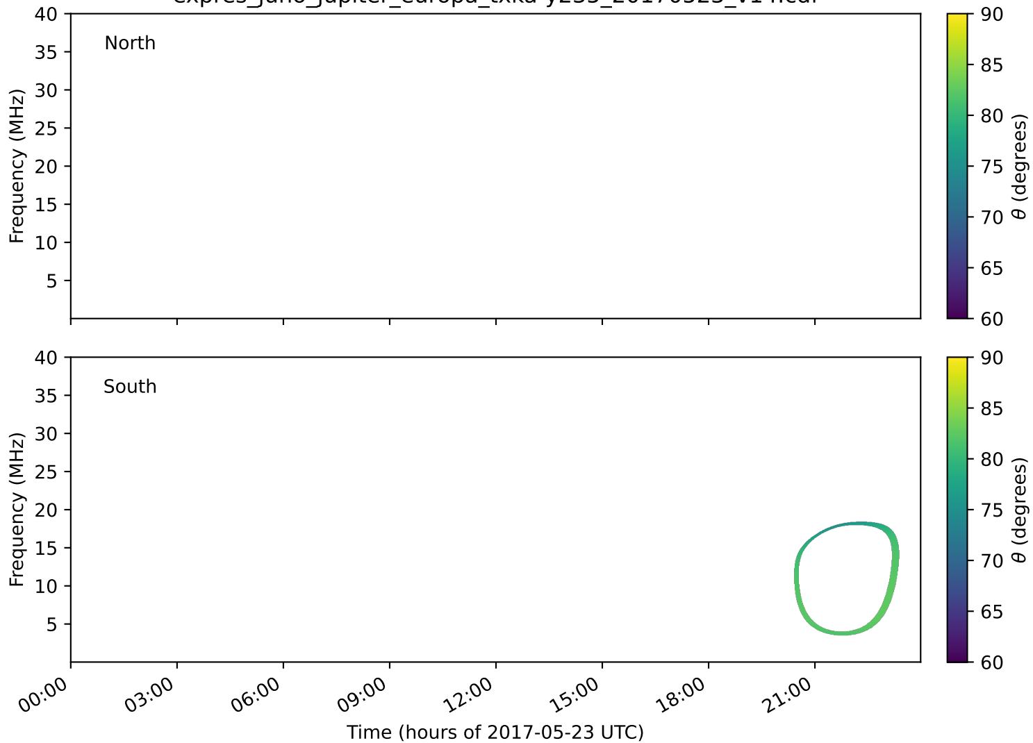
expres_juno_jupiter_europa_txka-y235_20170523_v14.cdf
