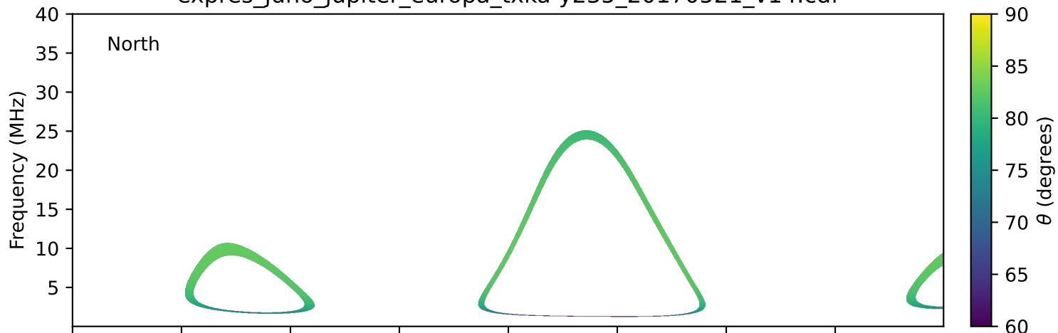
expres_juno_jupiter_europa_txka-y235_20170521_v14.cdf
