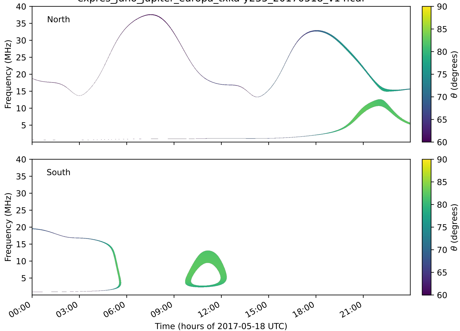
expres_juno_jupiter_europa_txka-y235_20170518_v14.cdf
