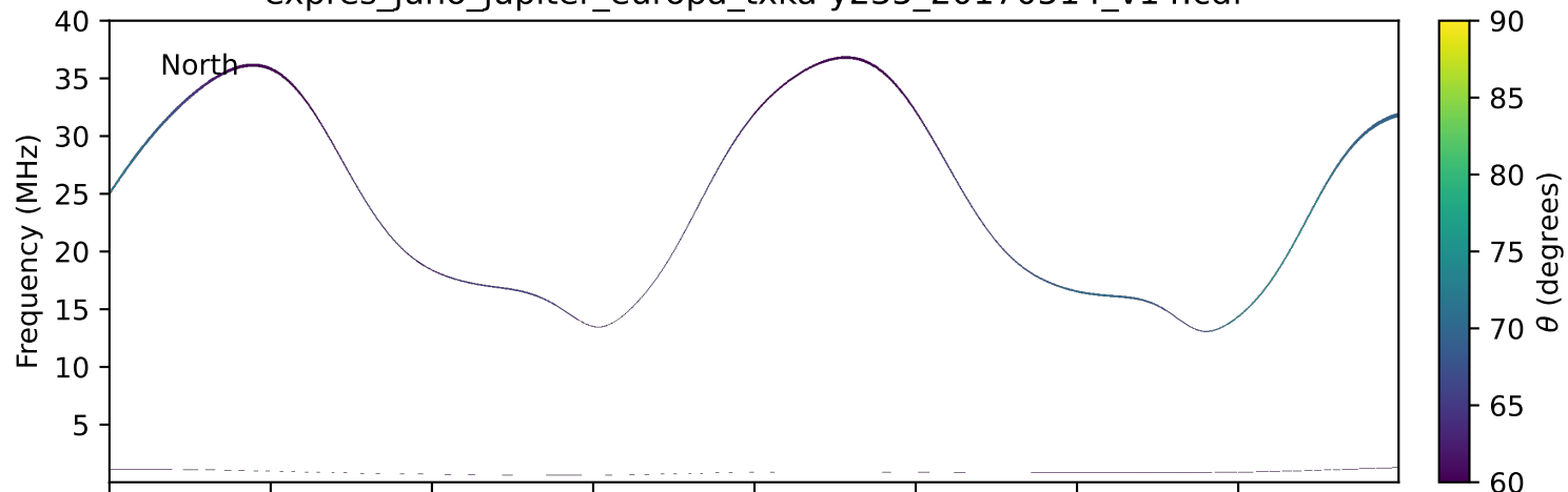
expres_juno_jupiter_europa_txka-y235_20170514_v14.cdf
