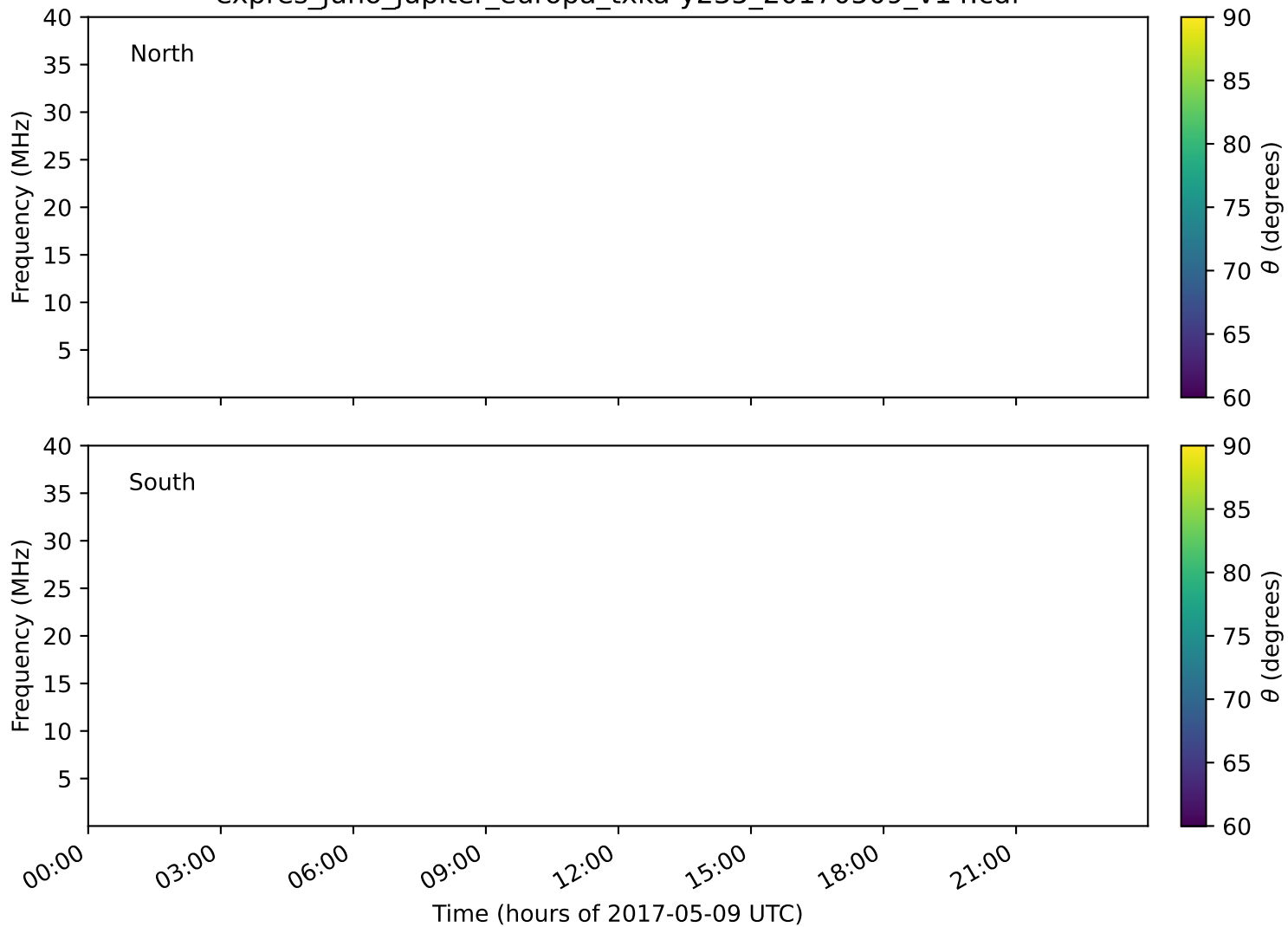
expres_juno_jupiter_europa_txka-y235_20170509_v14.cdf
