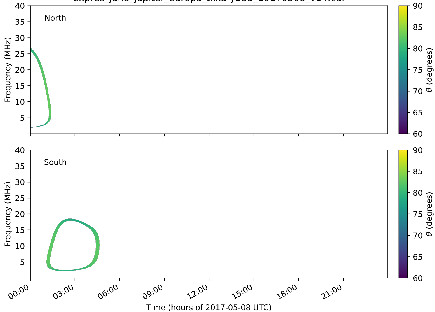
expres_juno_jupiter_europa_txka-y235_20170508_v14.cdf
