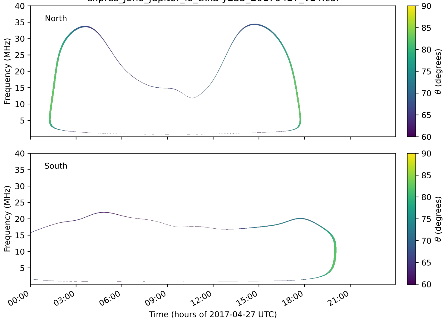
expres_juno_jupiter_io_txka-y235_20170427_v14.cdf
