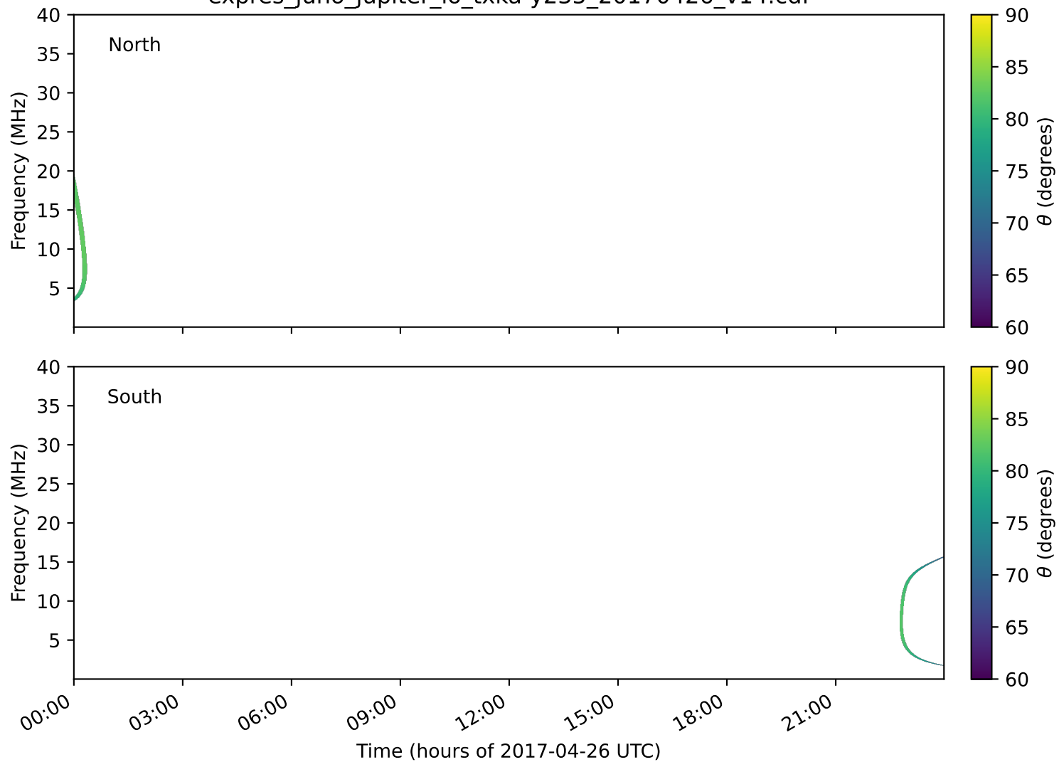
expres_juno_jupiter_io_txka-y235_20170426_v14.cdf
