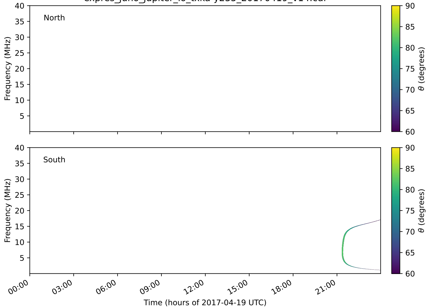
expres_juno_jupiter_io_txka-y235_20170419_v14.cdf
