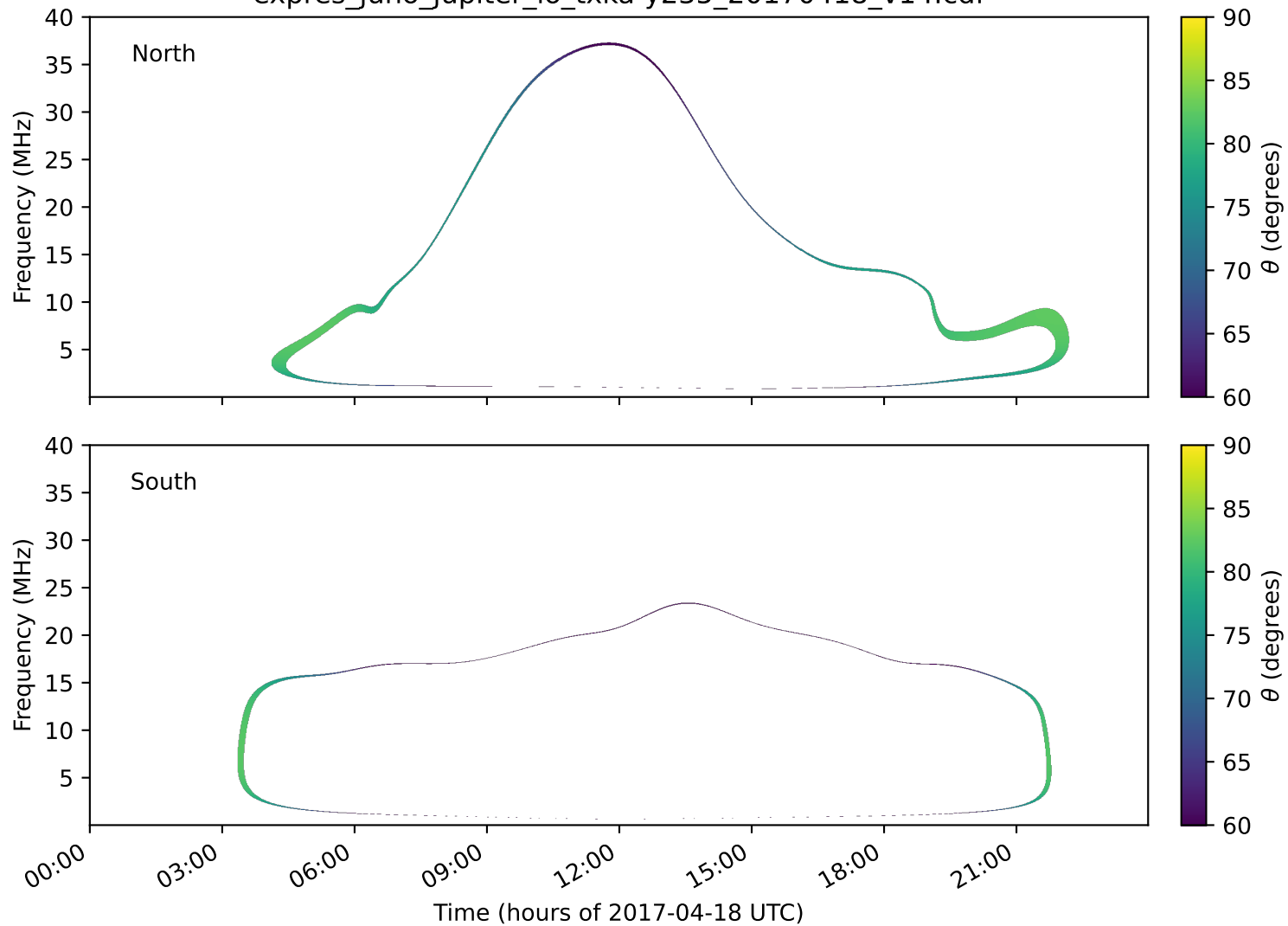
expres_juno_jupiter_io_txka-y235_20170418_v14.cdf
