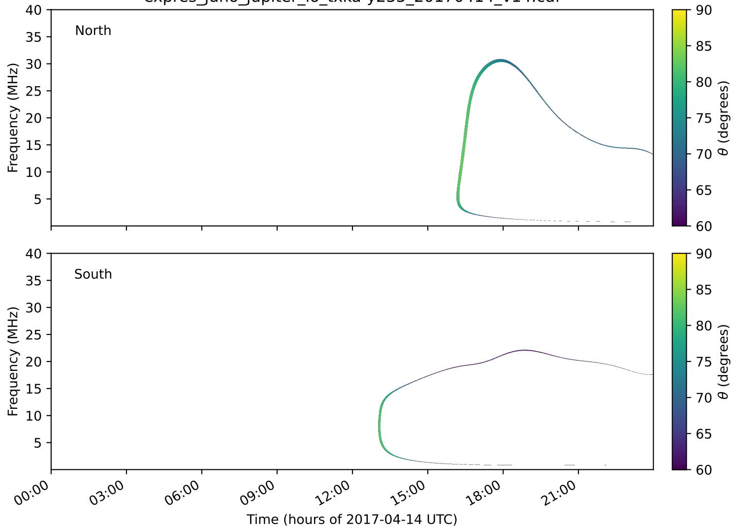
expres_juno_jupiter_io_txka-y235_20170414_v14.cdf
