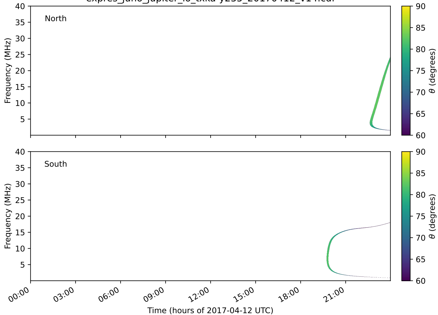
expres_juno_jupiter_io_txka-y235_20170412_v14.cdf
