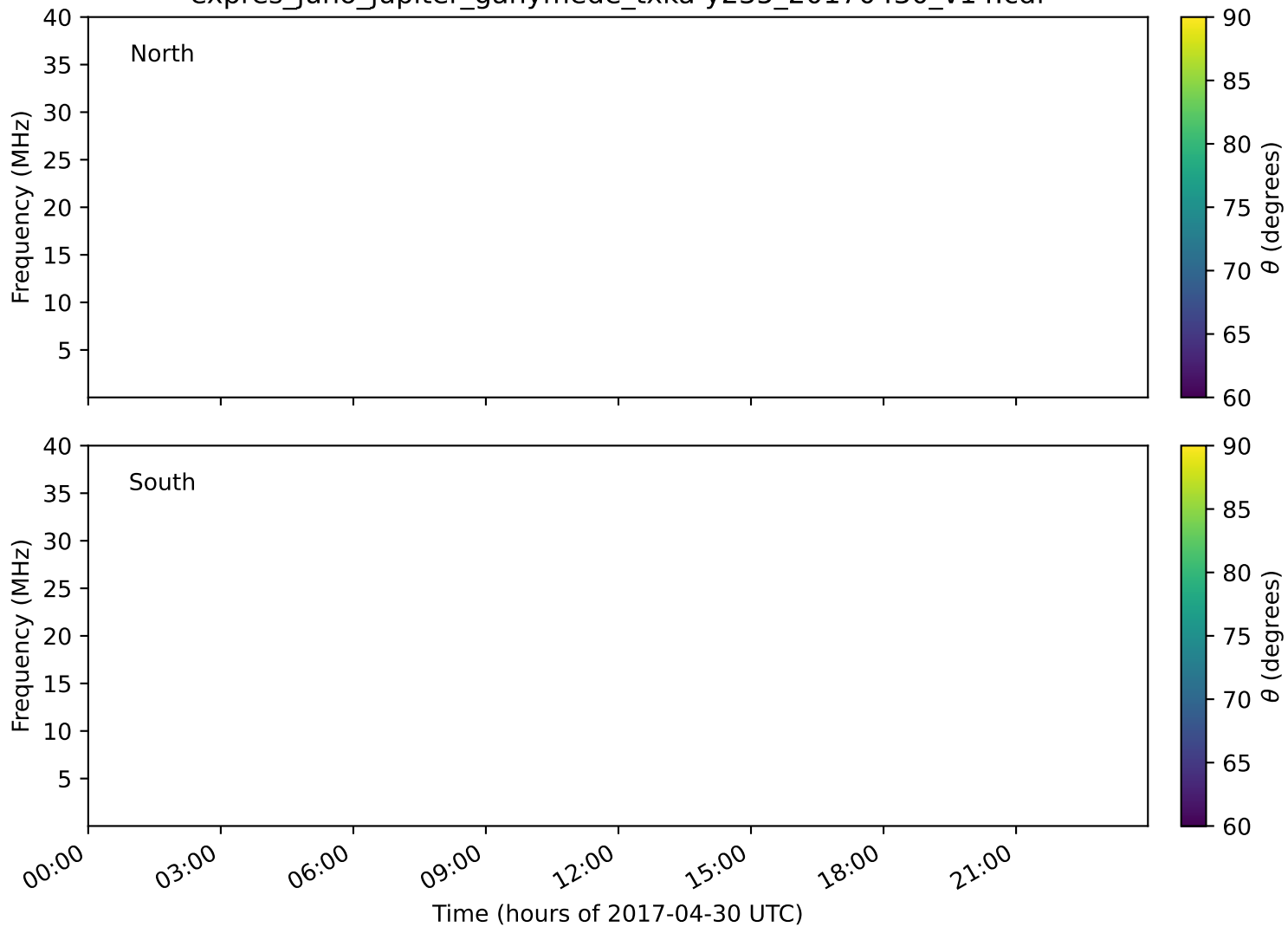
expres_juno_jupiter_ganymede_txka-y235_20170430_v14.cdf
