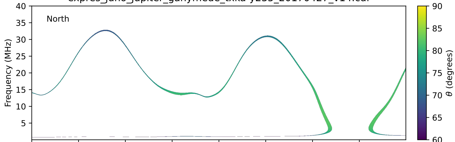
expres_juno_jupiter_ganymede_txka-y235_20170427_v14.cdf
