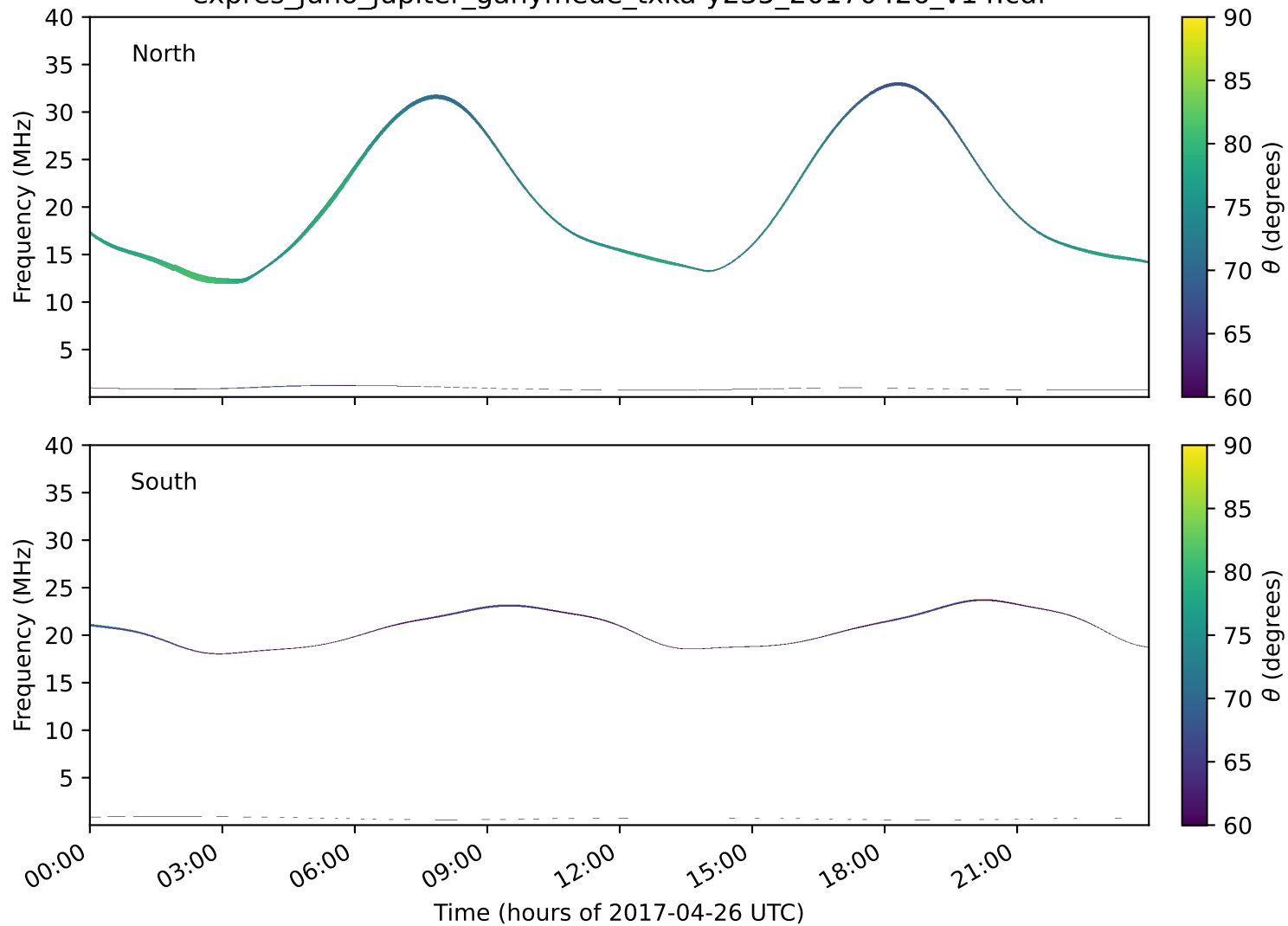
expres_juno_jupiter_ganymede_txka-y235_20170426_v14.cdf
