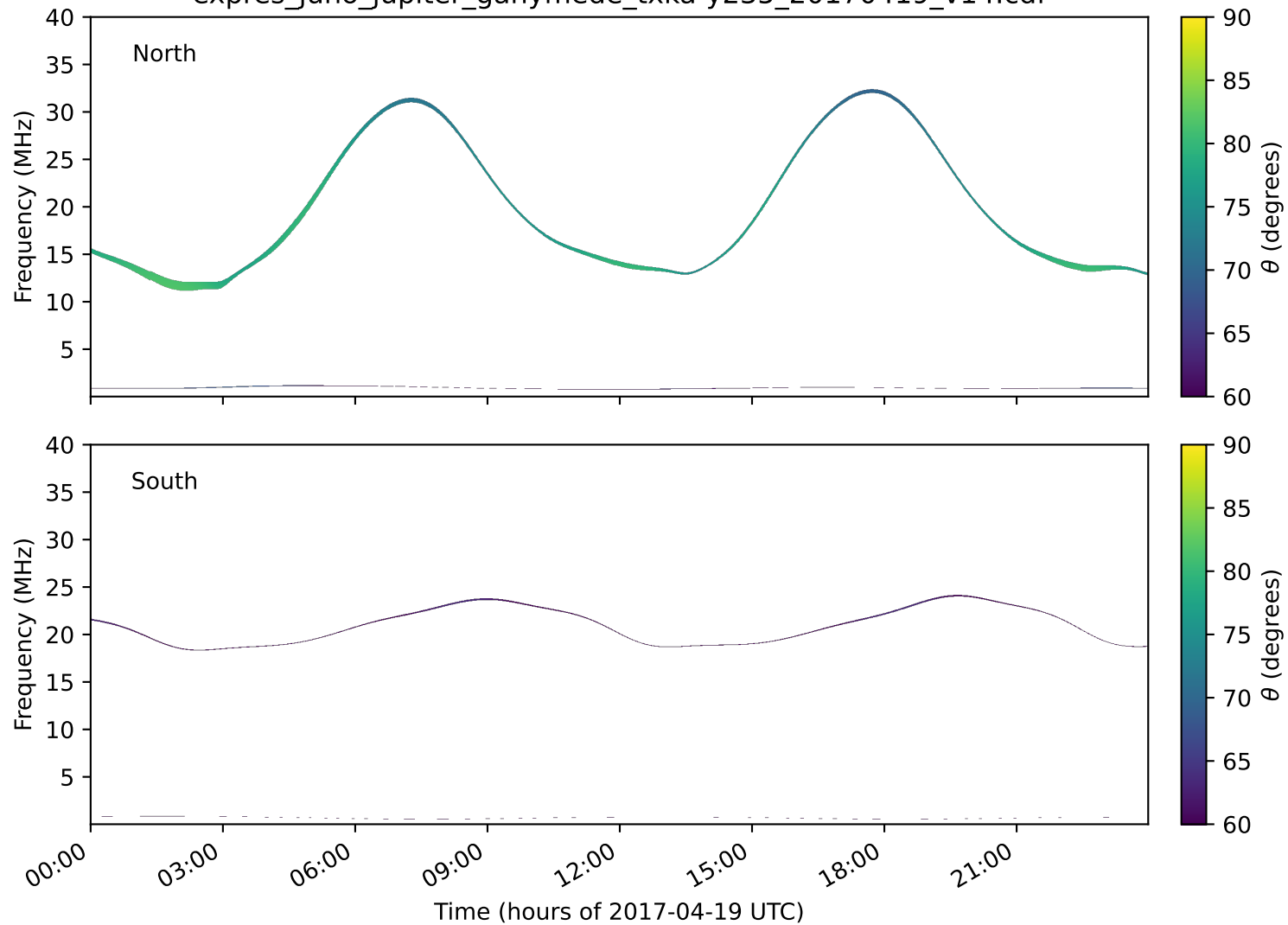
expres_juno_jupiter_ganymede_txka-y235_20170419_v14.cdf
