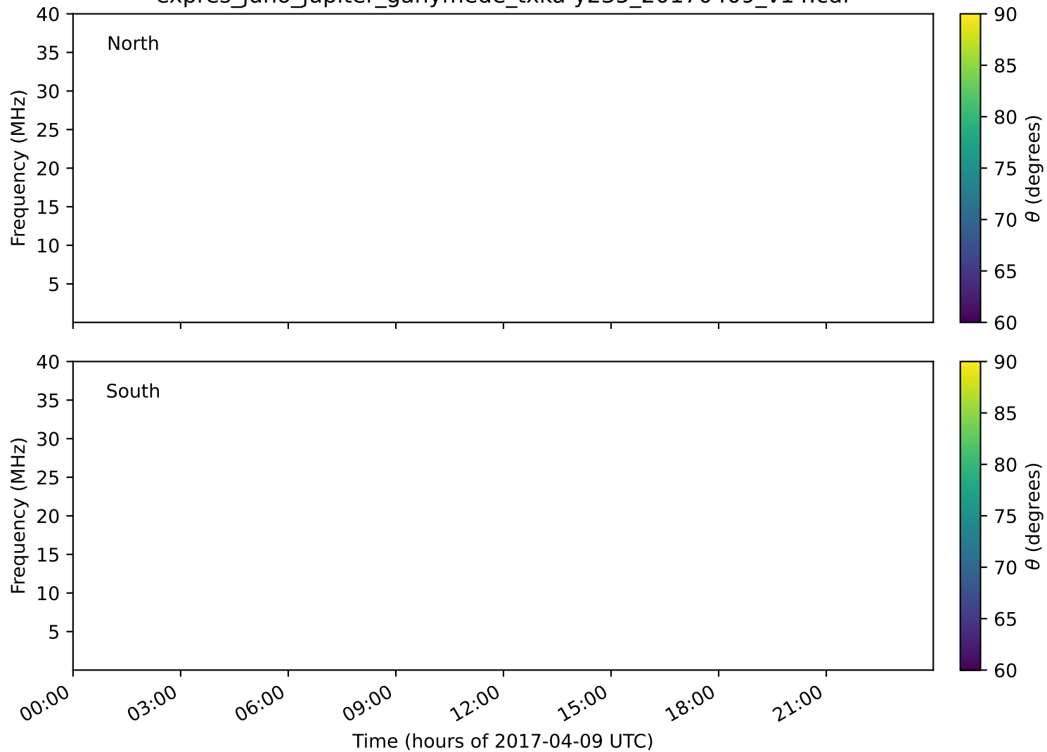
expres_juno_jupiter_ganymede_txka-y235_20170409_v14.cdf
