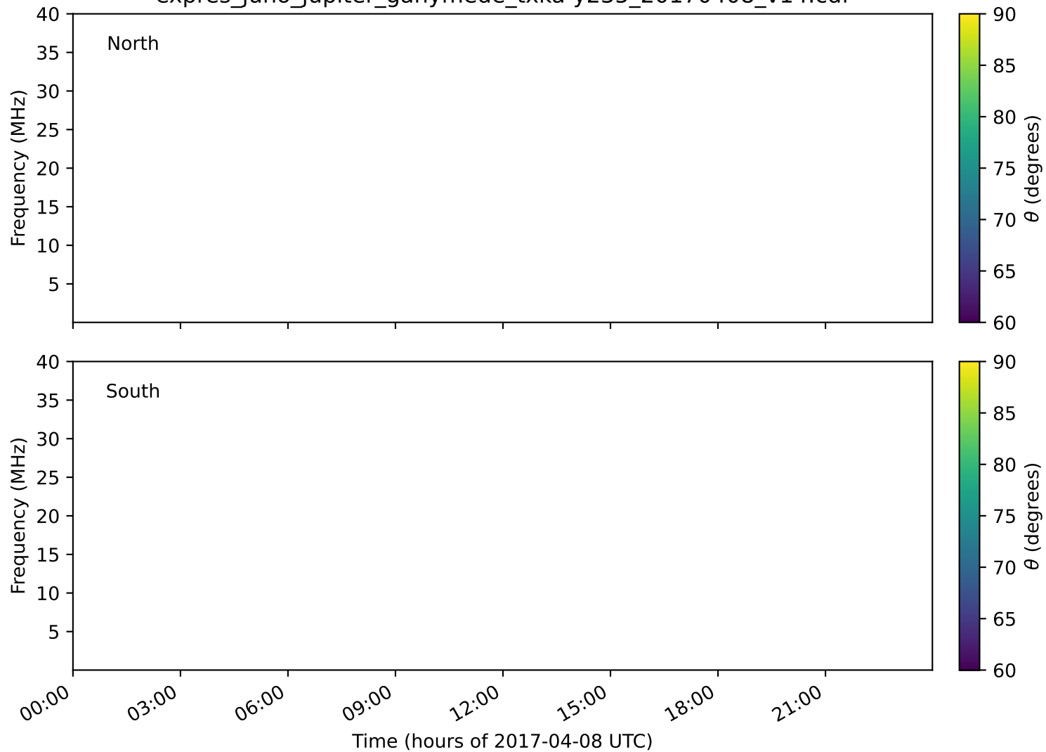
expres_juno_jupiter_ganymede_txka-y235_20170408_v14.cdf
