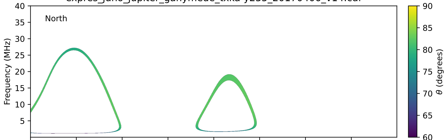
expres_juno_jupiter_ganymede_txka-y235_20170406_v14.cdf
