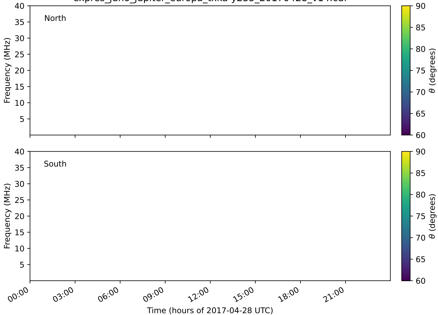
expres_juno_jupiter_europa_txka-y235_20170428_v14.cdf
