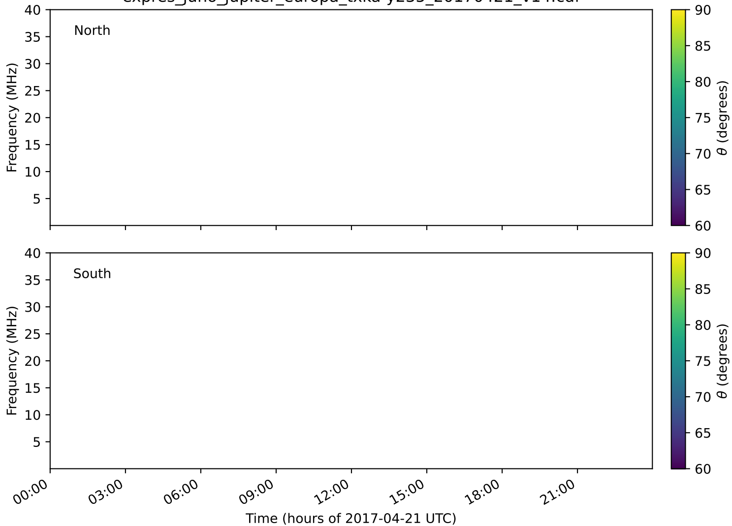
expres_juno_jupiter_europa_txka-y235_20170421_v14.cdf
