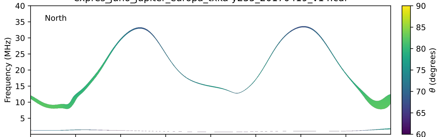
expres_juno_jupiter_europa_txka-y235_20170419_v14.cdf
