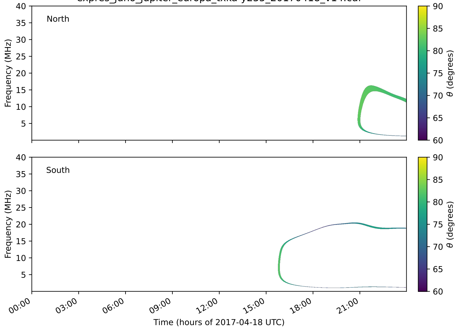
expres_juno_jupiter_europa_txka-y235_20170418_v14.cdf
