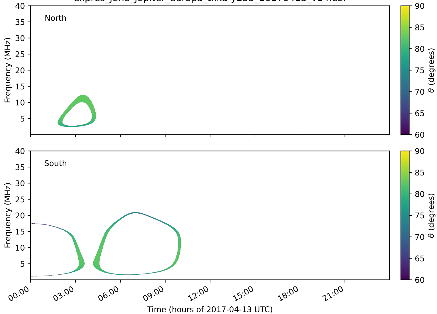
expres_juno_jupiter_europa_txka-y235_20170413_v14.cdf
