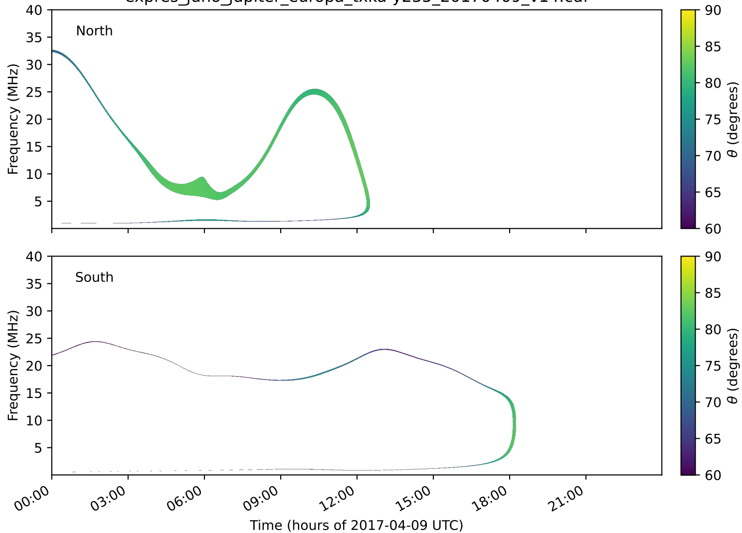
expres_juno_jupiter_europa_txka-y235_20170409_v14.cdf
