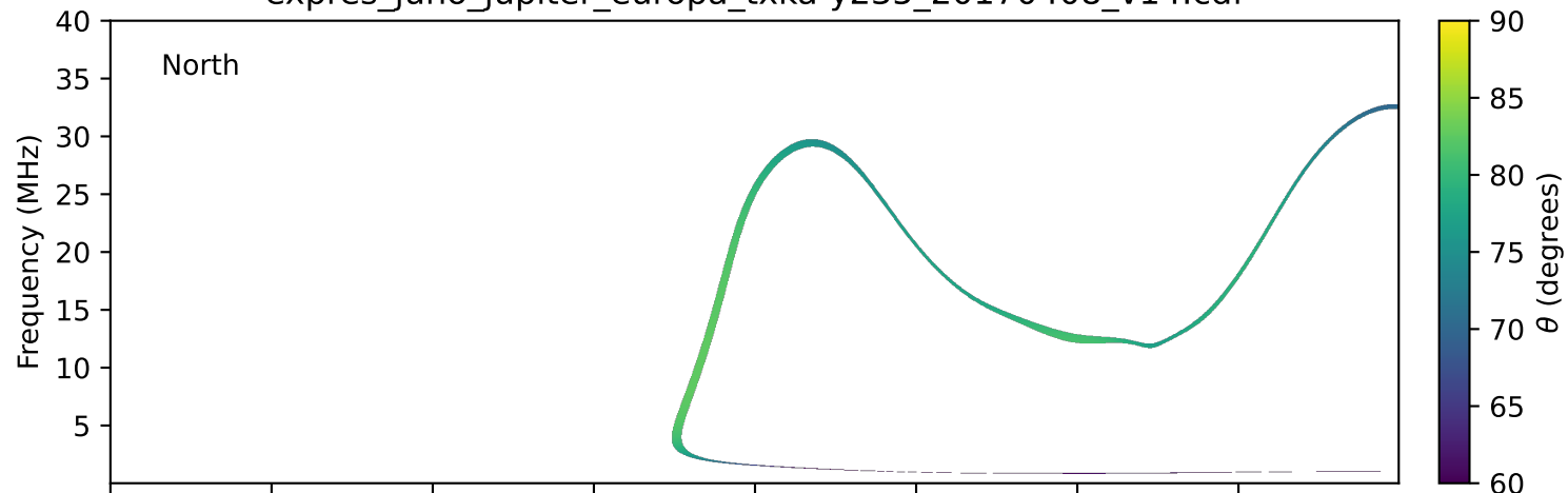
expres_juno_jupiter_europa_txka-y235_20170408_v14.cdf
