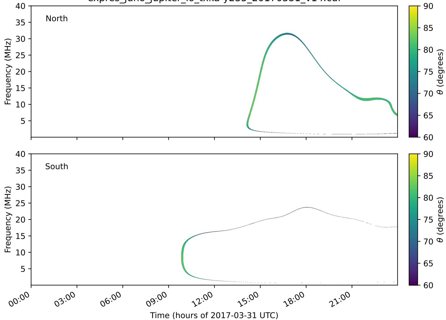
expres_juno_jupiter_io_txka-y235_20170331_v14.cdf
