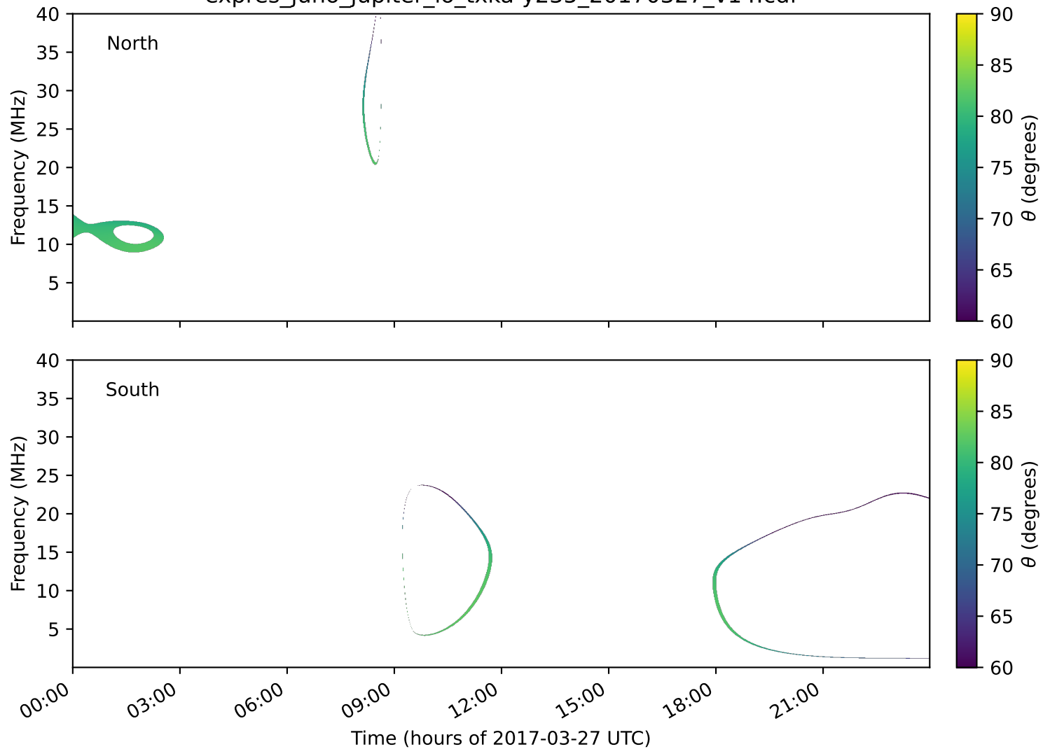
expres_juno_jupiter_io_txka-y235_20170327_v14.cdf
