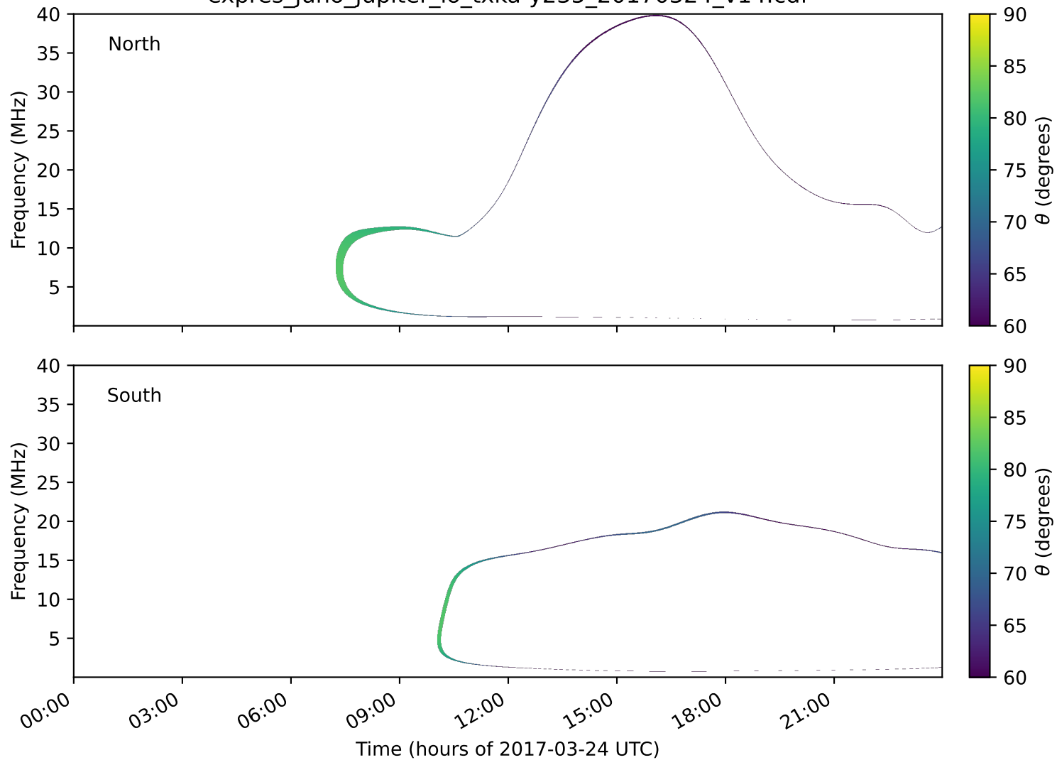
expres_juno_jupiter_io_txka-y235_20170324_v14.cdf
