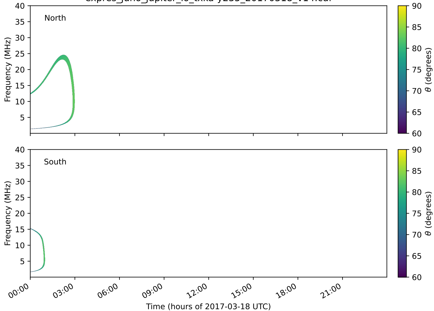
expres_juno_jupiter_io_txka-y235_20170318_v14.cdf
