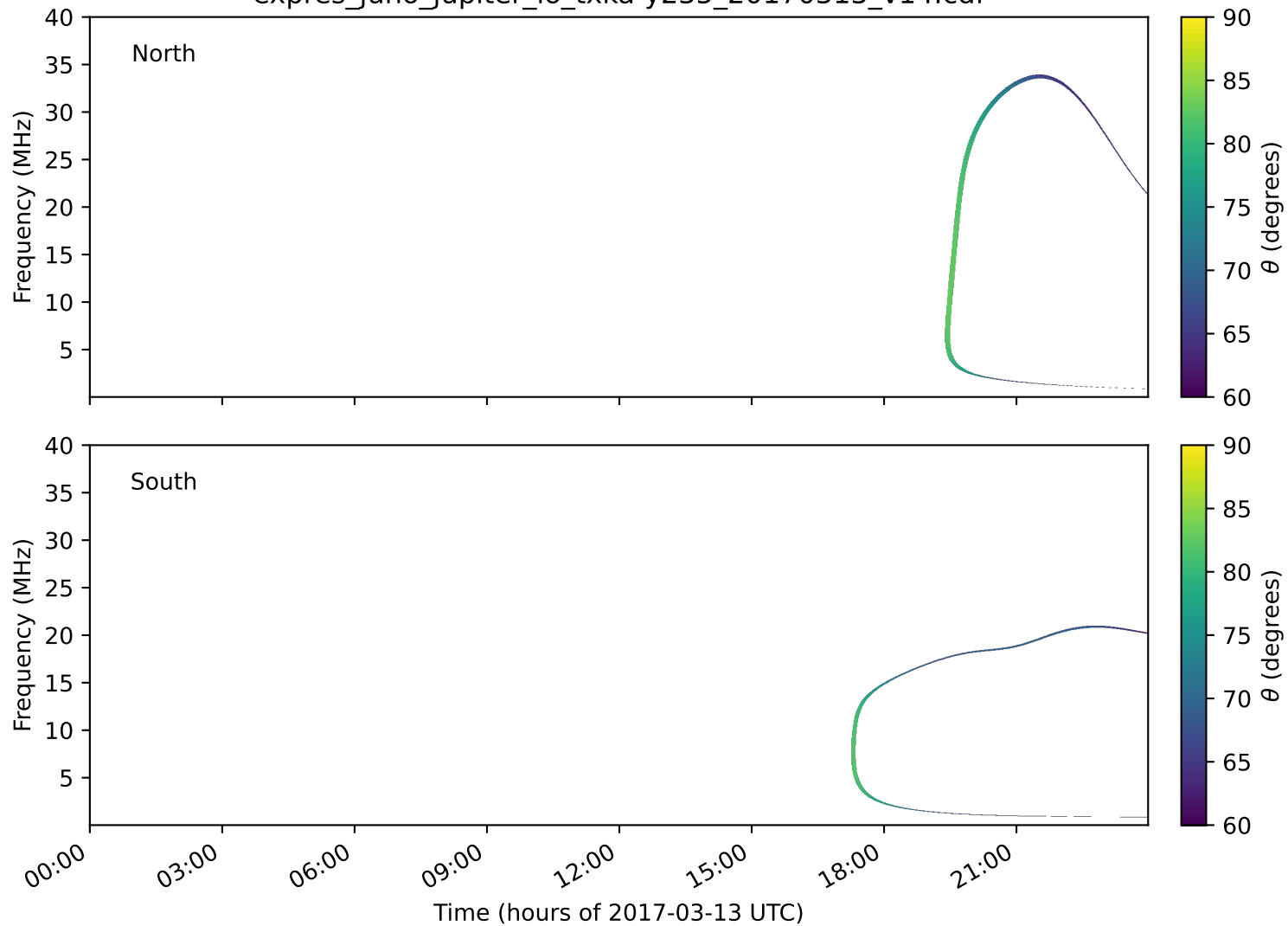
expres_juno_jupiter_io_txka-y235_20170313_v14.cdf
