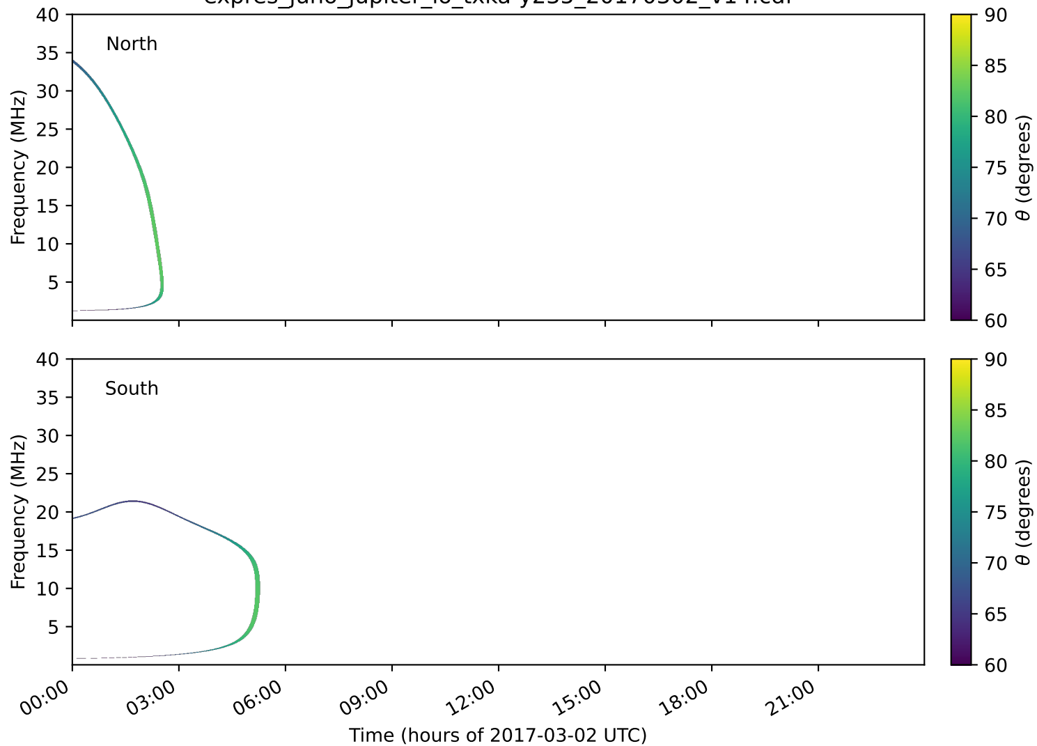
expres_juno_jupiter_io_txka-y235_20170302_v14.cdf
