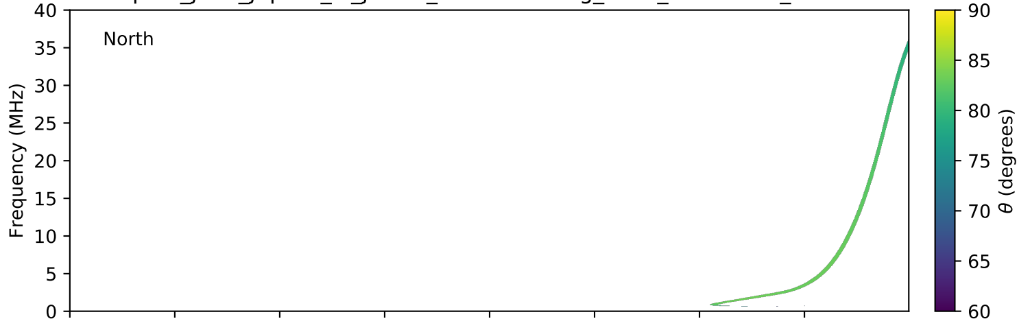
expres_juno_jupiter_io_jrm09_lossc-wid1deg_3kev_20170329_v01.cdf
