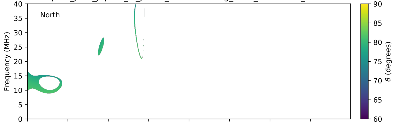
expres_juno_jupiter_io_jrm09_lossc-wid1deg_3kev_20170327_v01.cdf
