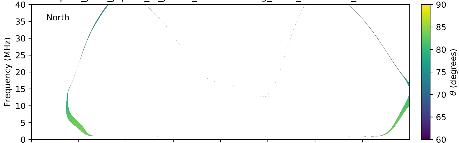
expres_juno_jupiter_io_jrm09_lossc-wid1deg_3kev_20170326_v01.cdf
