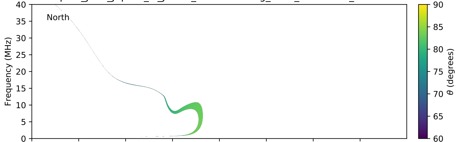
expres_juno_jupiter_io_jrm09_lossc-wid1deg_3kev_20170323_v01.cdf
