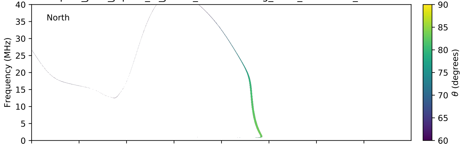
expres_juno_jupiter_io_jrm09_lossc-wid1deg_3kev_20170321_v01.cdf
