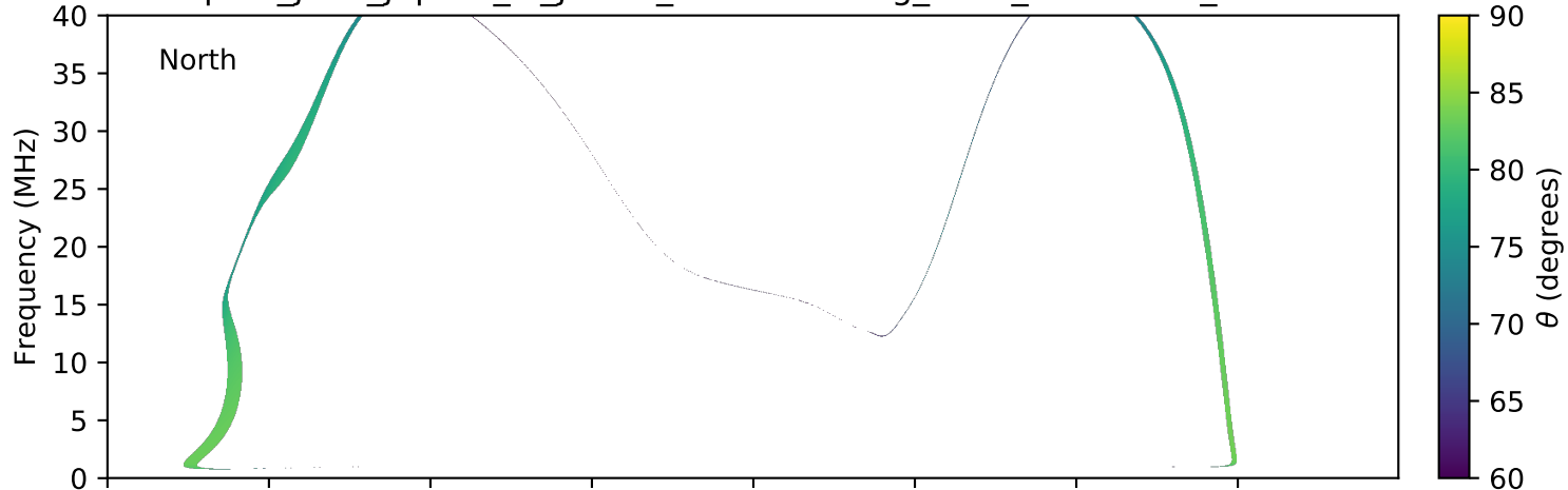
expres_juno_jupiter_io_jrm09_lossc-wid1deg_3kev_20170319_v01.cdf
