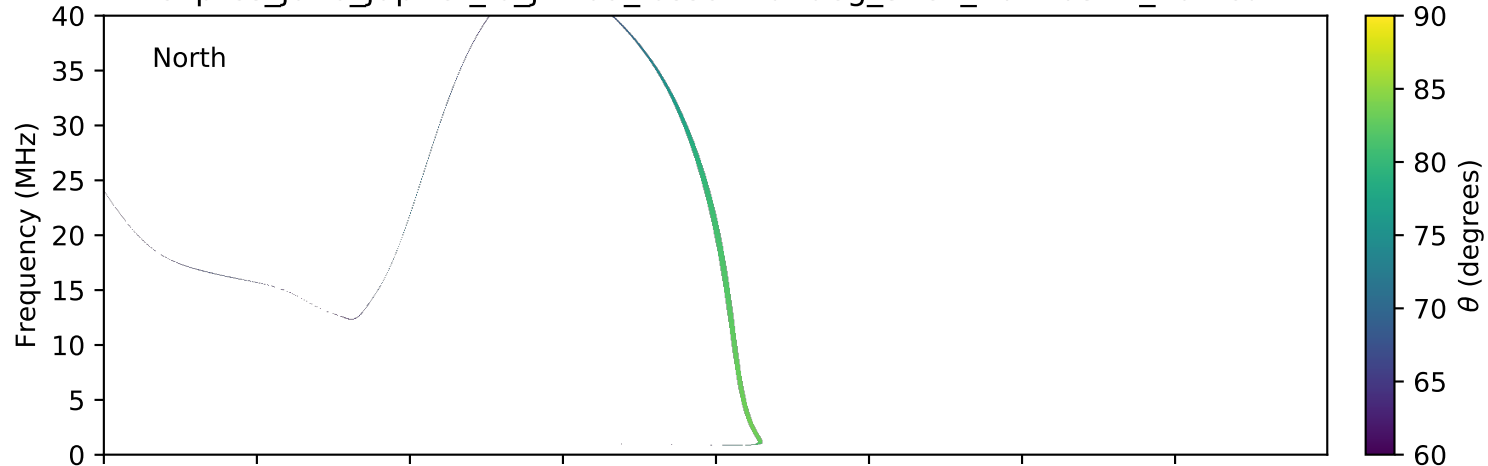
expres_juno_jupiter_io_jrm09_lossc-wid1deg_3kev_20170314_v01.cdf
